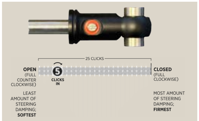
12. The FOX ATS Direct Fit Grenadier Steering Stabilizer by Agile Offroad is equipped with a slotted adjustment screw on the passenger side eyelet that affects steering damping. Turning the adjustment screw clockwise will increase damping, making the steering firmer, while adjusting counterclockwise will decrease damping and steering resistance. **The stabilizer comes factory set at 5 clicks from open. This is the recommended starting point**
