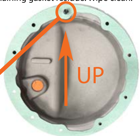
Place supplied gasket onto AO Diff Cover with letter side facing cover and blank side facing differential. Install one bolt in top hole.
